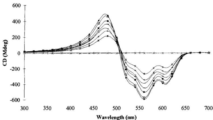
Figure 5. Circular Dichroism spectra of 1 in chloroform-methanol solutions. (x) 100% \text{CHCl}_3 , (*) 55% \text{CHCl}_3 , (+) 54% \text{CHCl}_3 , (-) 53% \text{CHCl}_3 , (-) 52%, (■) 50% \text{CHCl}_3 , (□) 47% \text{CHCl}_3 , (◆) 39% \text{CHCl}_3 .
