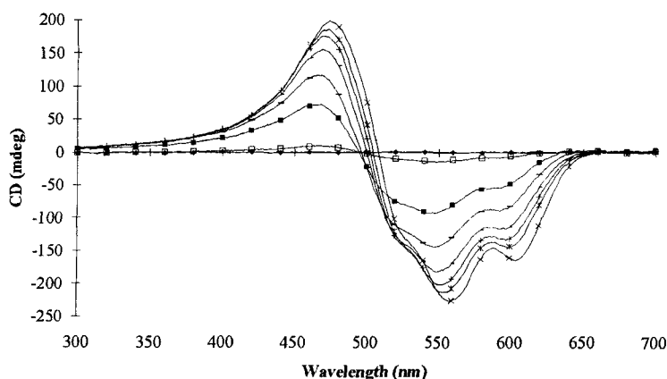
Figure 7. Temperature dependence of the Circular Dichroism of 1 . (x) 20°C, (*) 50°C, (+) 60°C, (-) 70°C, (—) 80°C, (■) 90°C, (□) 100°C, (◆) 110°C.
